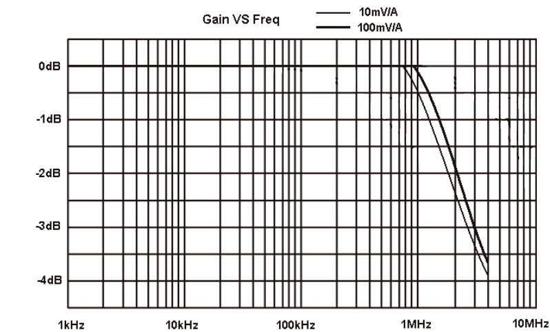
Figure 1: Bandwidth
